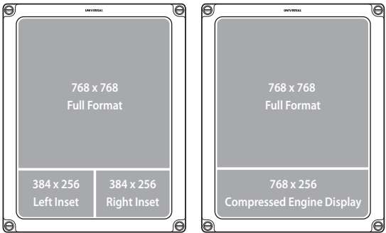
PFD with Insets
